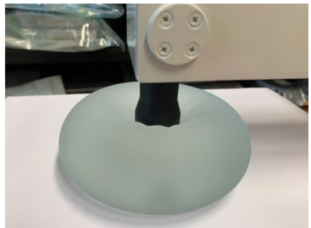
Fig. 1: Indentation test of breast implant.
